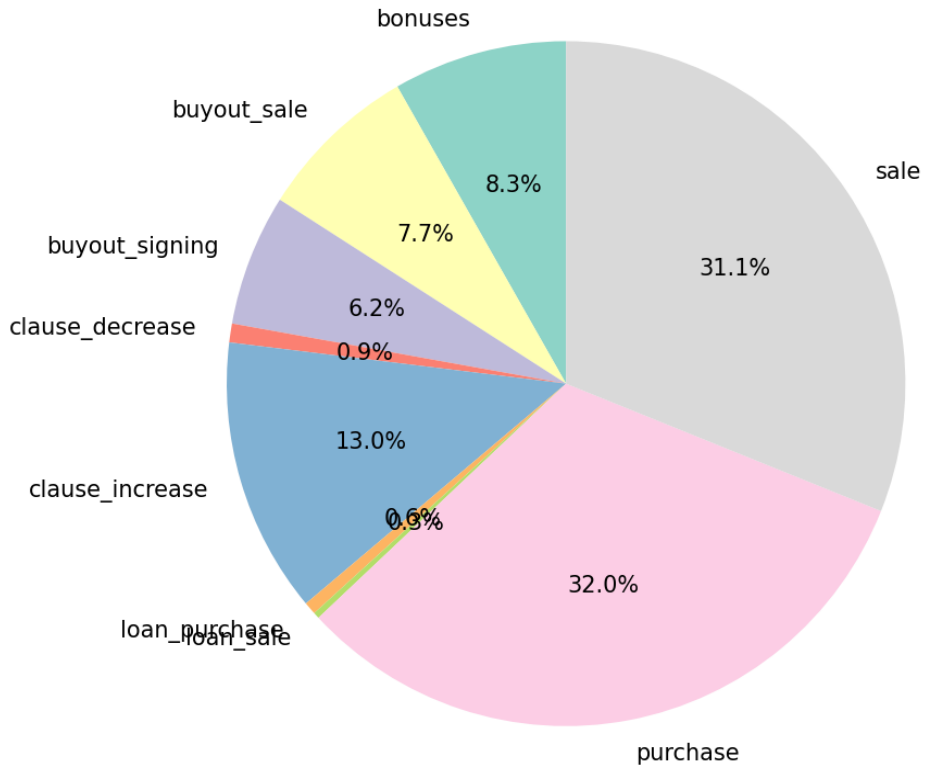
Transaction Distribution
